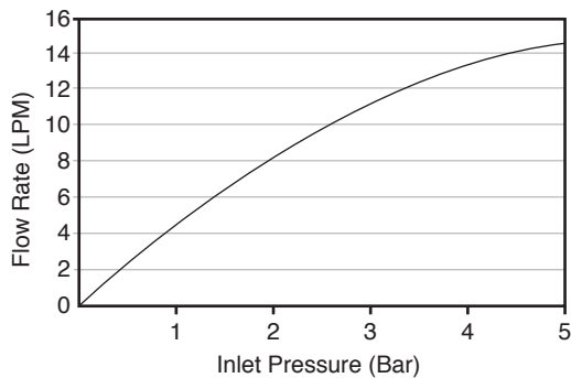
Flow Curve - K-9302
